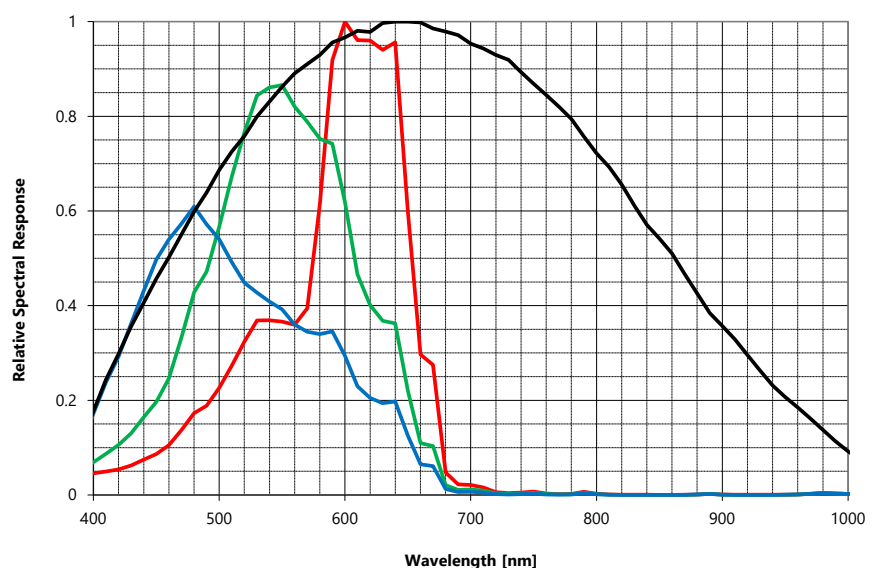
FASTCAM Nova R2 Relative Spectral Response Curves - Monochrome and Color
